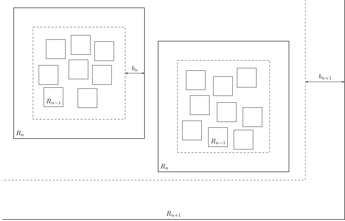
FIGURE 6. Rokhlin towers
