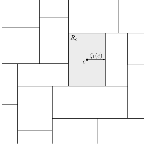
FIGURE 3. Rectangular tiling
