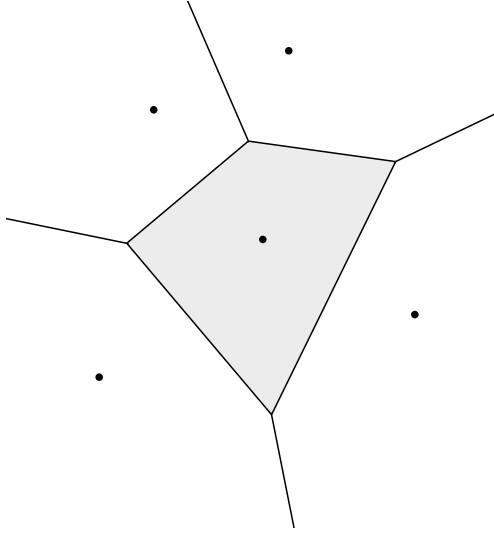
FIGURE 2. Voronoi tessellation
